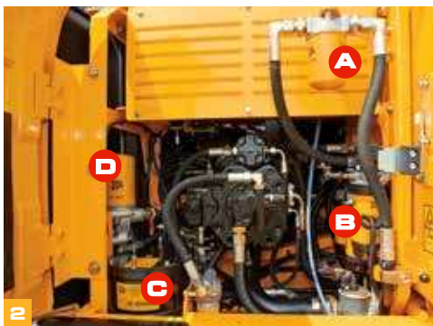
(A) Hydraulics oil filters (B) Fuel filters (C) JCB Plexus Oil Filter System (D) Engine Oil Filter
