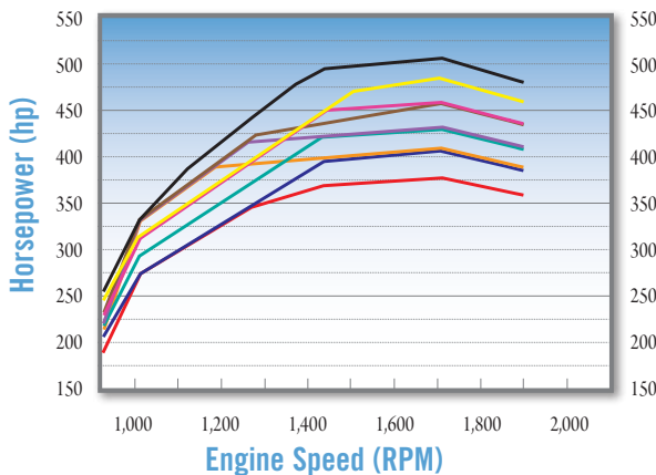
Horsepower
