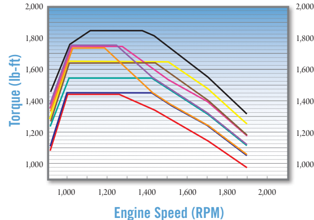
Torque
