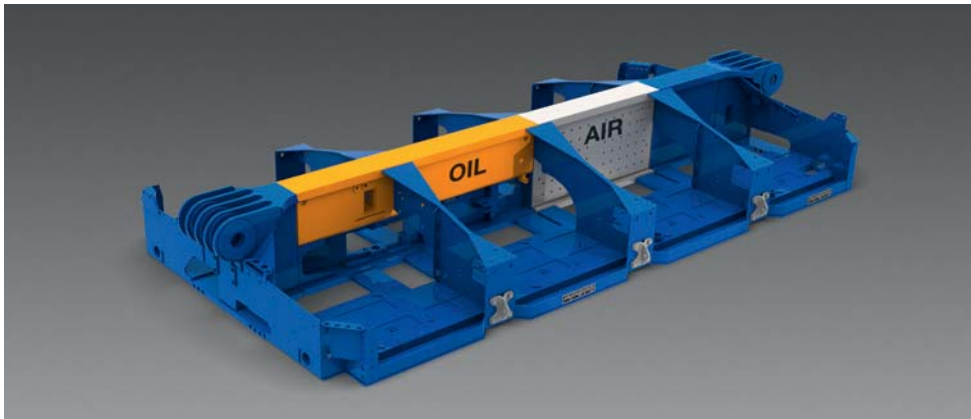
Center beam in box-section design with integrated compressed air and hydraulic oil tanks
