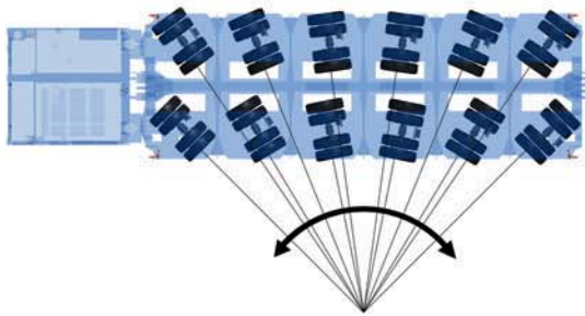
1. Counter steering
