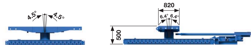
300 T/400 T TURNTABLE
