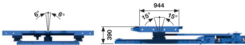
100 T/200 T TURNTABLE
