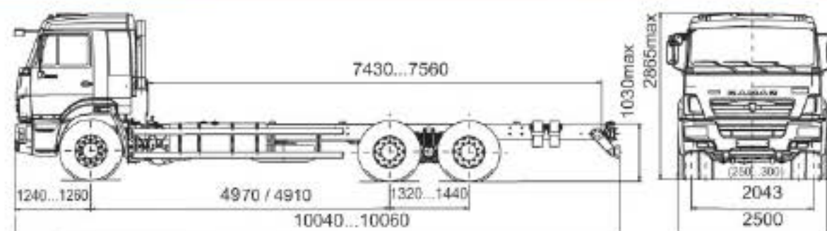
Dimensions with curb (gross) weight 4910+1440 mm wheelbase is used in modifications with the rear air suspension
