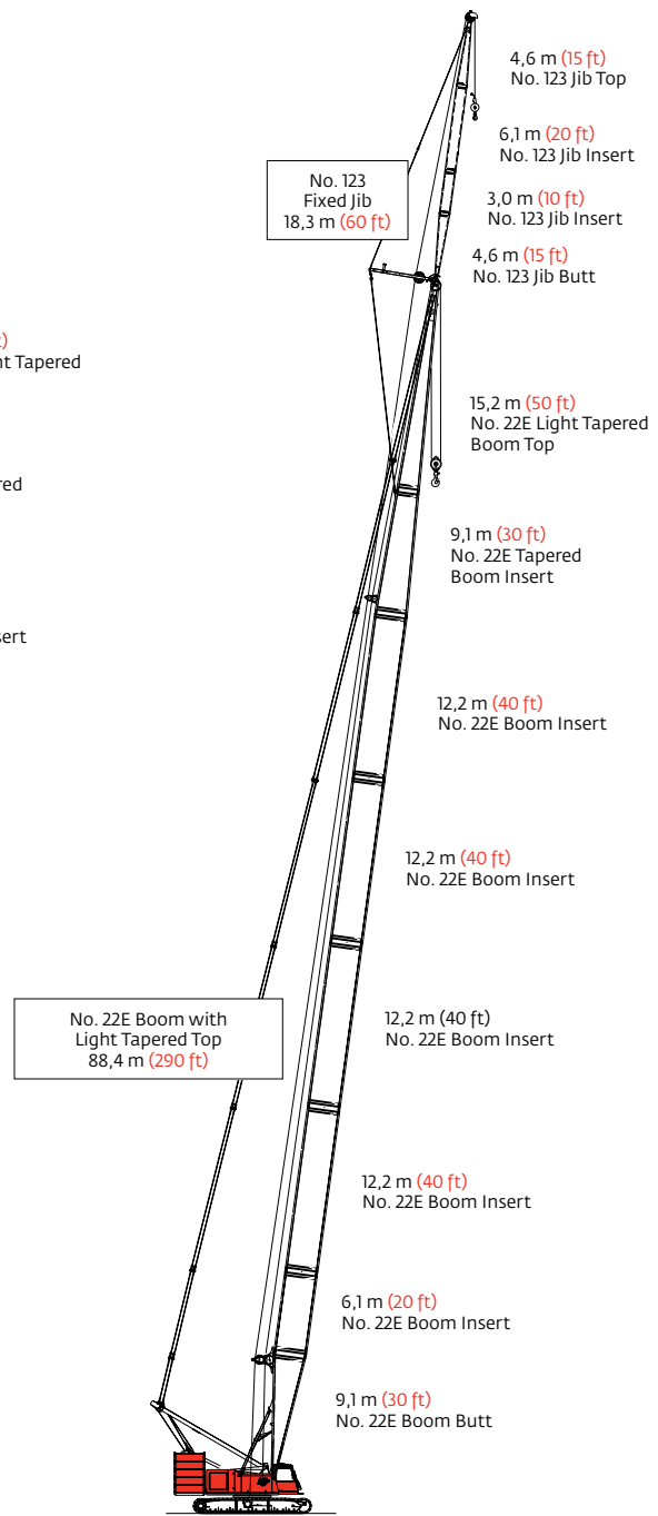
Model 999 Series 3 No. 123 Fixed Jib on No. 22E Boom with Light Tapered Top 106,7 m (350 ft)
